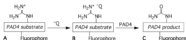
Scheme 1. The fluorescent PAD4 substrate A forms a nonfluorescent noncovalent complex B with a negatively charged quencher dye molecule. Upon citrullination of the PAD4 substrate, the now neutral product C loses its affinity for the dye, and a fluorescence response is observed.
