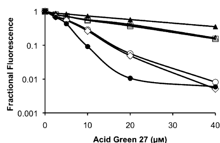
Figure 1. Fractional fluorescence of Cit-containing TAMRA-GlyXaaGly-AlaGlyXaaGlyAlaGlyXaaGlyAla derivatives as a function of Acid Green 27 concentration. Fractional fluorescence = fluorescence in the presence versus the absence of Acid Green 27. Xaa in TAMRA-GlyXaaGly-AlaGlyXaaGlyAlaGlyXaaGlyAla: Arg...Arg...Arg (●); Arg...Arg...Cit (◊); Cit...Arg...Arg (○); Cit...Cit...Arg (□); Arg...Cit...Cit (Δ); Cit...Cit...Cit (▲).
